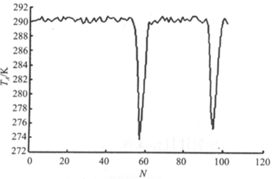
图6 辐射计偏离混凝土物160米时的仿真计算结果 Fig.6 Digital simulating results when the radiometer is far from the concrete target by 160 meter
