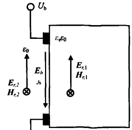
Fig.1 PCSS in biased electric field 图1 电场偏置的PC器件
