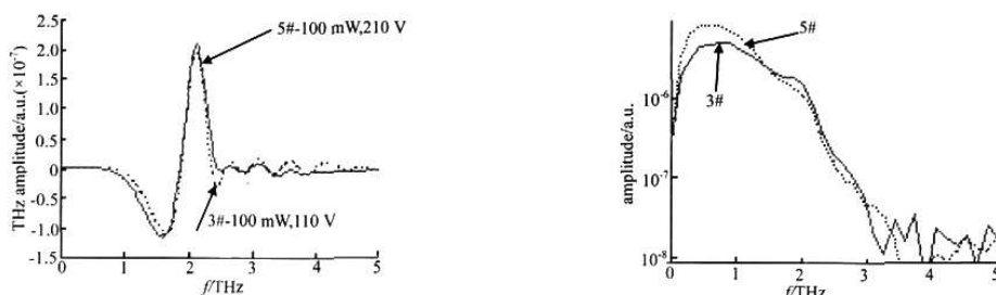
Fig.6 THz time domain waveform and frequency of rectangle PCA with different gaps
