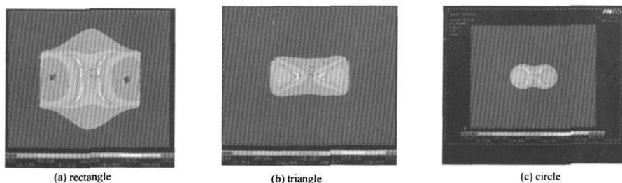
Fig.3 Current distribution planform of different electrode shapes 图3 电场强度分布俯视图
