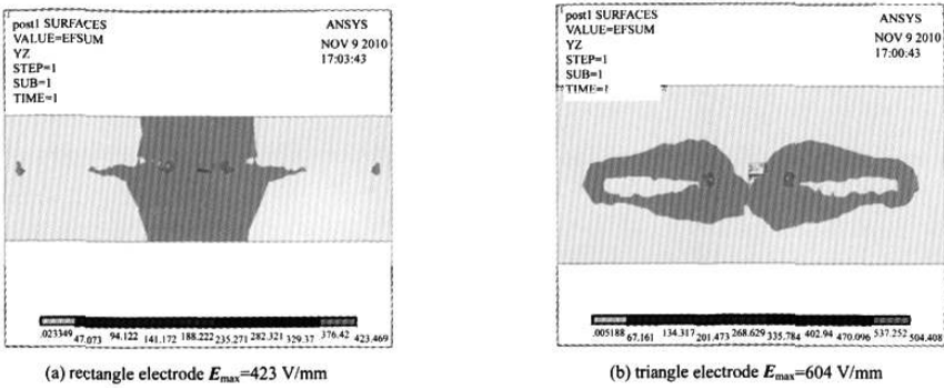
Fig.4 Current distribution section of rectangle and triangle electrodes 图 4 中轴线电场分布剖面图
