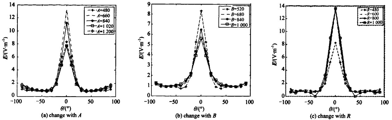
Fig.8 Plot of the radiated pattern in the vertical H -plane for the IRA in time domain when the aperture of the TEM horn lies in the focus of the reflector 图 8 喇叭口面位于焦点处时 H 面时域方向图
