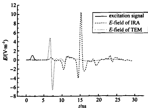
Fig.4 Plot of the excitation waveform and radiation field of IRA and TEM 图 4 信号波形及辐射波形图
