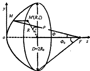
Fig.1 The IRA geometry and coordinate system 图 1 抛物面几何结构
