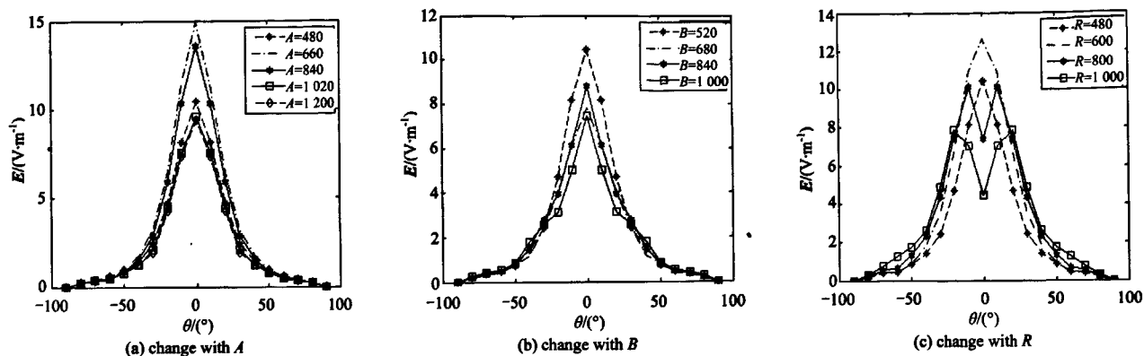
Fig.5 Plot of the radiated pattern in the vertical E -plane for the IRA in time domain when the plane of the transmission line and plate lie in the focus of the reflector
