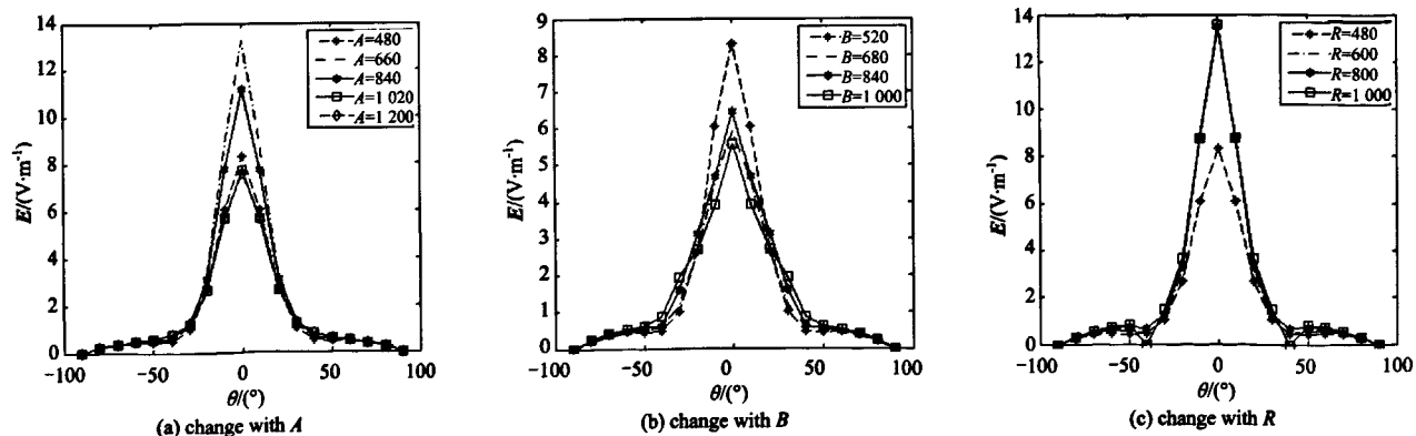
Fig.7 Plot of the radiated pattern in the vertical E -plane for the IRA in time domain when the aperture of the TEM horn lies in the focus of the reflector
