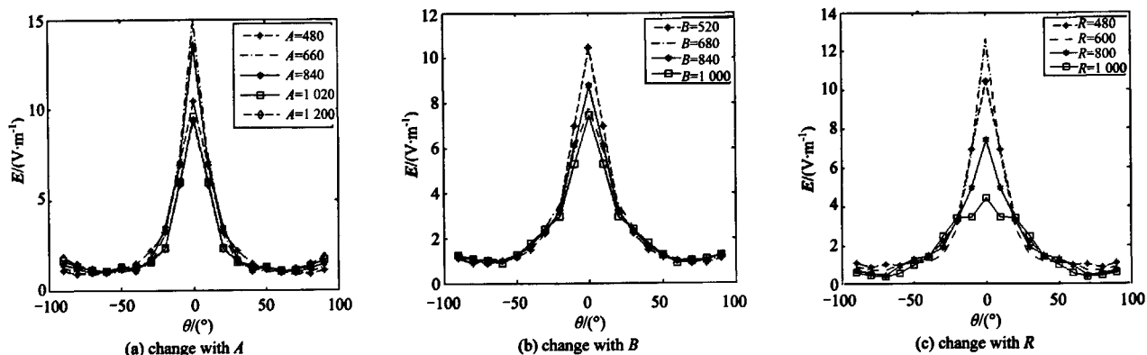
Fig.6 Plot of the radiated pattern in the vertical H -plane for the IRA in time domain when the plane of the transmission line and plate lie in the focus of the reflector
