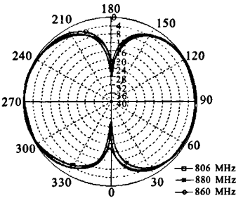
图 6 天线 E 面归一化辐射方向图(低频段) Fig. 6 The normalized radiation pattern in E-plane(low frequency band)
