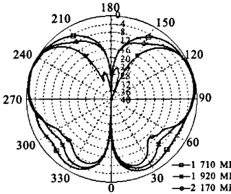
图 7 天线 E 面归一化辐射方向图(中频段) Fig. 7 The normalized radiation pattern in E-plane(middle frequency band)
