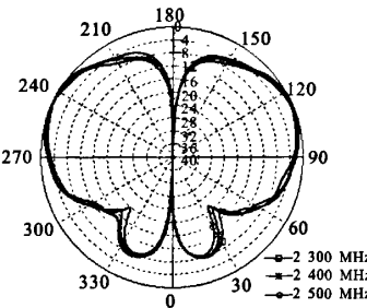
图 8 天线 E 面归一化辐射方向图(高频段) Fig. 8 The normalized radiation pattern in E-plane(high frequency band)
