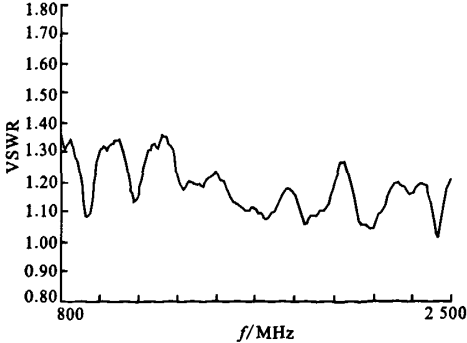
图5 天线电压驻波比(实测) Fig. 5 VSWR(actual measurement)
