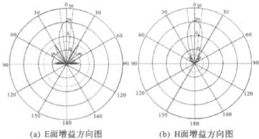
图 12 加载零折射率超材料喇叭天线的增益方向图(7.1 GHz) Fig. 12 Gain patterns of the horn antenna with ZIM at 7.1 GHz
