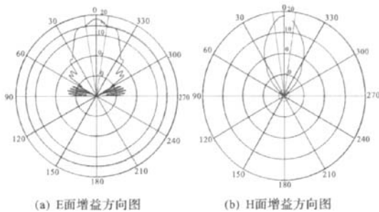
图 9 喇叭天线的增益方向图(7.1 GHz) Fig. 9 Gain patterns of the horn antenna at 7.1 GHz
