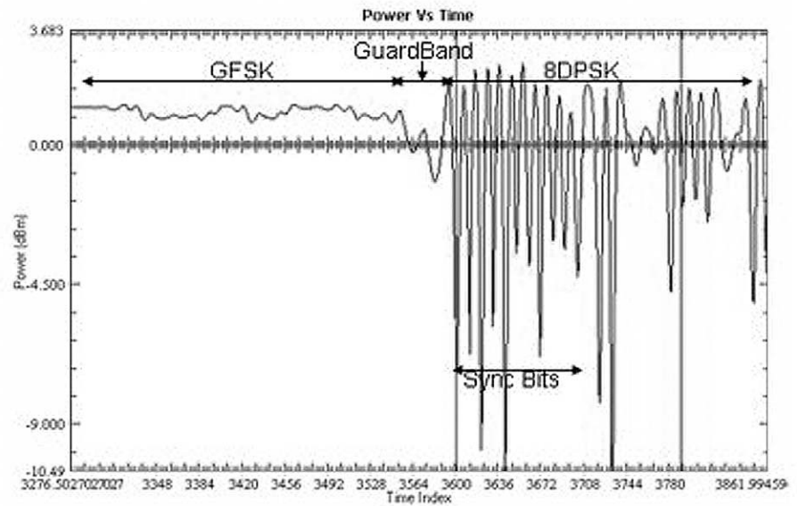
Figure 5b. Power versus time waveform displaying the transition between GFSK and 8DPSK modulation schemes
