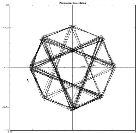
Figure 6. Measurement constellation of an EDR payload using a \pi/4 -DQPSK modulation
