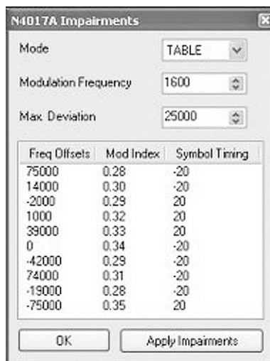
Figure 12. Agilent N4017A signal impairments menu for creating dirty packets in an EDR waveform
