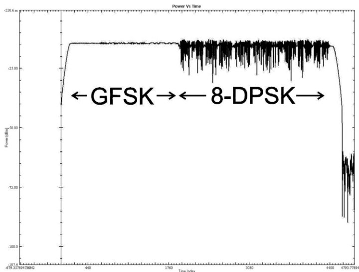
Figure 5a. Power versus time measurement for an EDR packet showing the GFSK and 8-DPSK modulated sections of the packet.) This waveform was captured using the Agilent N4017A Graphical Measurement Application (GMA) with Option 205 for Bluetooth EDR testing)
