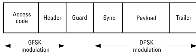
Figure 4. Bluetooth EDR packet format
