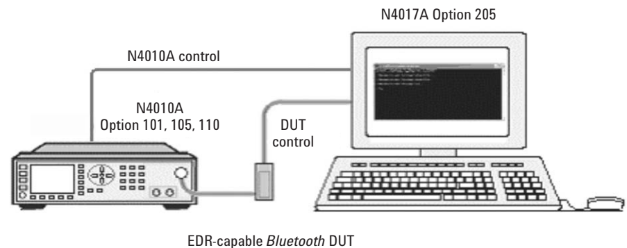
Figure 7. Measurement configuration for testing a Bluetooth EDR radio using the Agilent N4010A test set and N4017A Graphical Measurement Application
