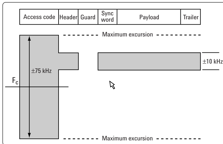
Figure 10. Bluetooth EDR carrier frequency stability limits as a function of the symbol position
