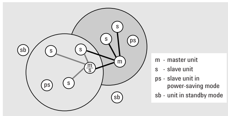
Figure 1. Scatternet topology formed by two piconets sharing common devices
