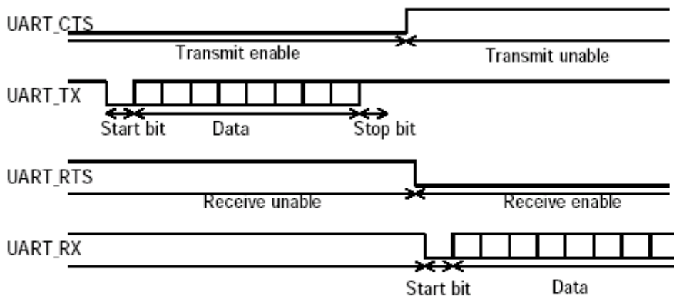
UART timing chart (No parity, 1 Stop bit)
