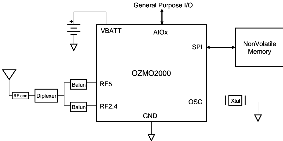
Figure 1 Wireless Module Block Diagram (battery not included)
