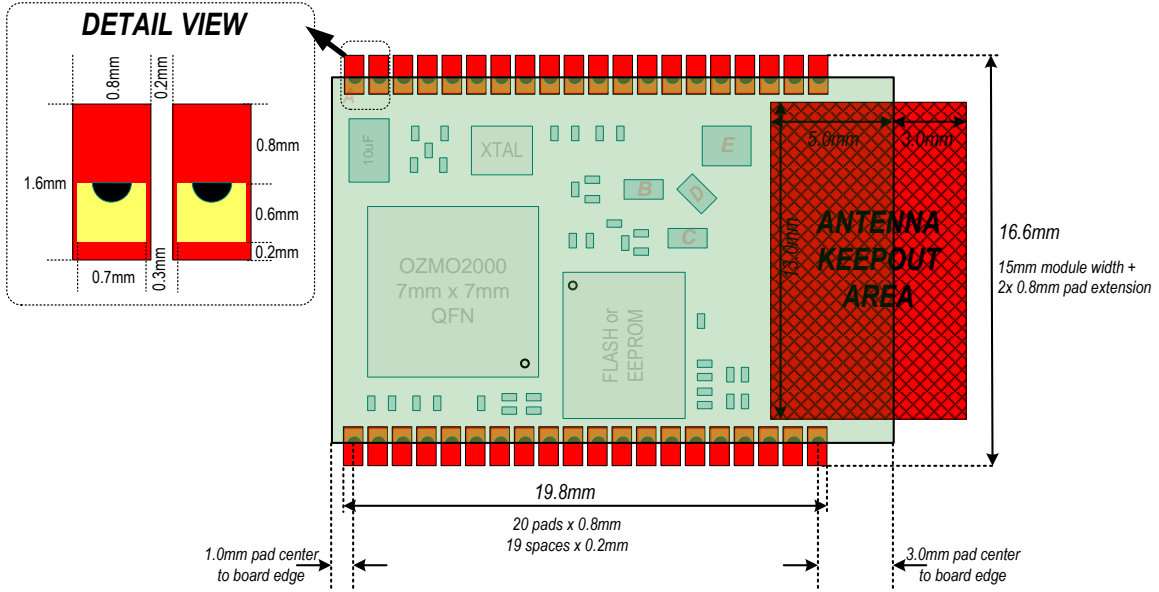
Figure 3 Host PCB footprint for OZMO2000 Wireless Module
