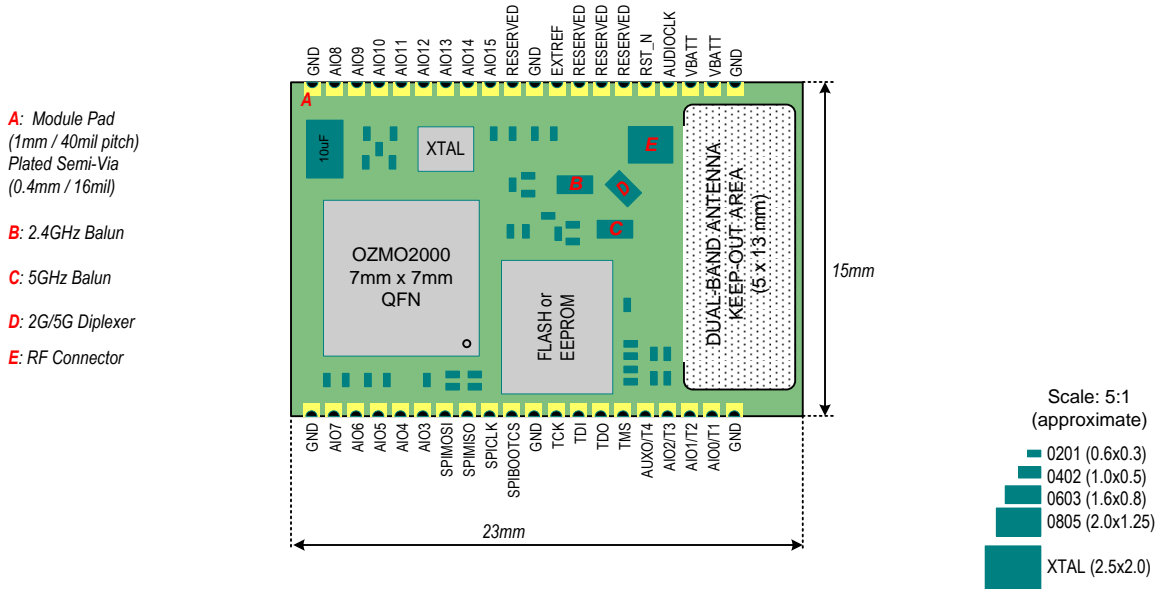
Figure 2 Floorplan of the OZMO2000 Wireless Module
