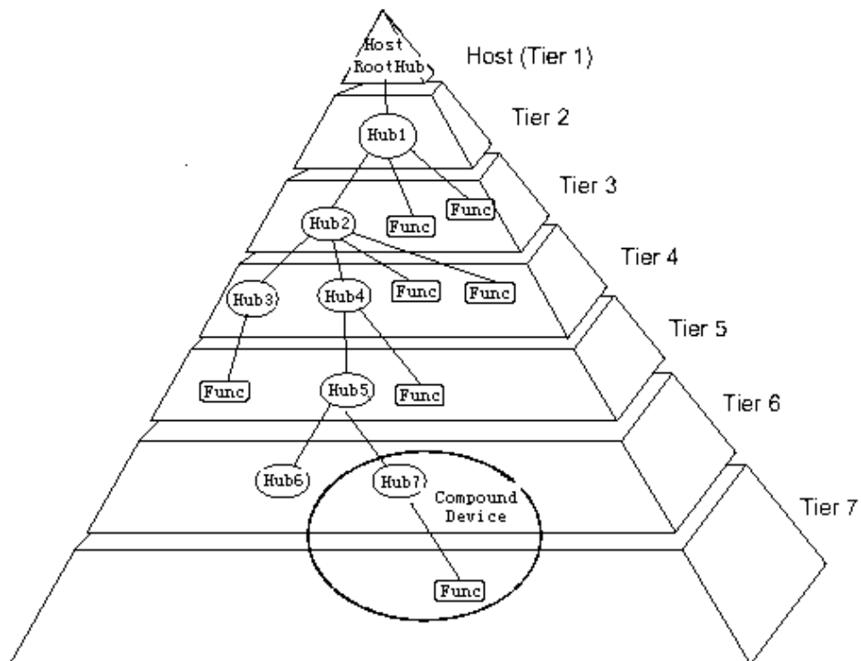
图 1: USB Toplogy
