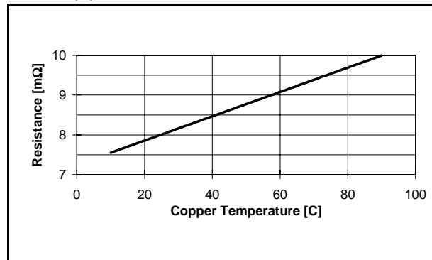
Figure 2. Resistance vs Copper Temperature for Example Design
