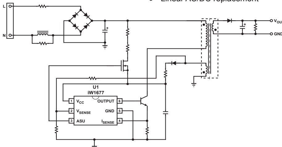
Figure 3.1: iW1677 Typical Application Circuit
