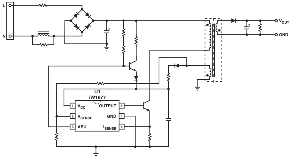
Figure 3.2: iW1677 Typical Application Circuit
